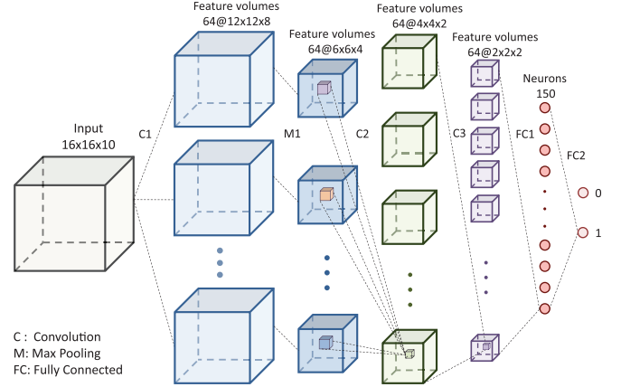
Fig. 4. The hierarchical architecture of the 3D CNN model.
